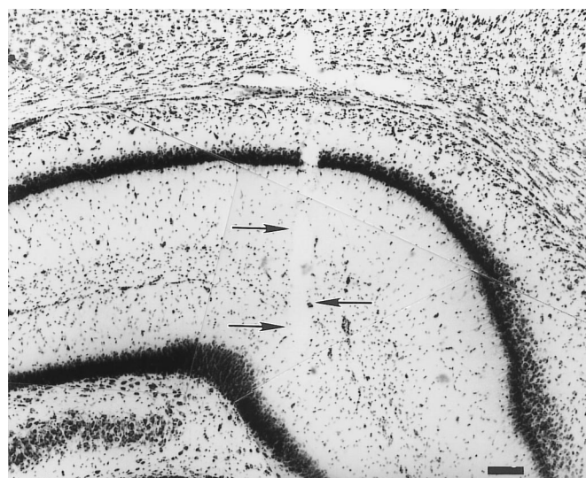
FIG. 7. Location of area CA1/subiculum stimulation site used for in vivo activation of the entorhinal cortex. Stimulation site used for the recordings shown in Fig. 6 is illustrated in a montage of adjacent Nissl-stained sections from the brain that was used for that experiment. Note the track made by the stimulating electrode ( \rightarrow ) passes into area CA1 near the subiculum. Only 1 pole of the electrode is shown in this section; the other pole was in a similar area in a more anterior section. Scale bar, 100 \mu\text{m} .
